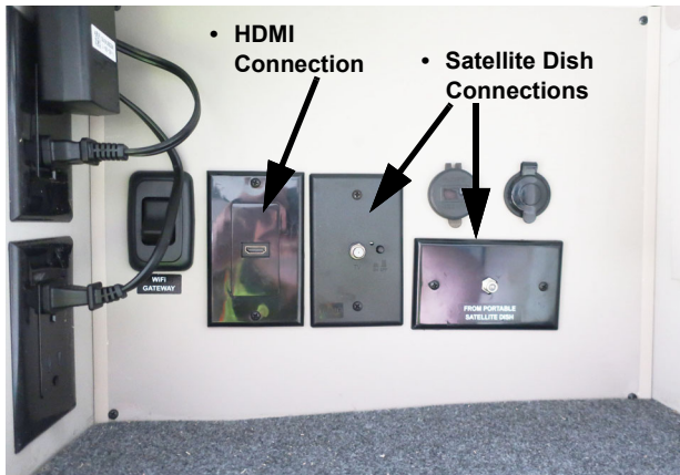
Interior Satellite Dish and HDMI Connections (Located near entertainment center cabinet) -Typical installation shown- configuration may vary.
